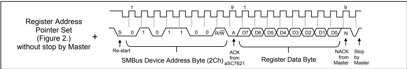
Figure 4 Register Read
