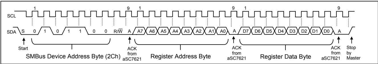
Figure 3 Register Write
